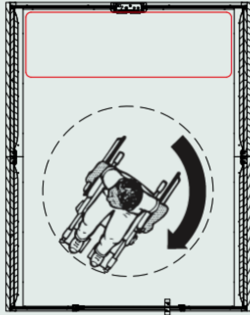
Circular space in hushFree.Access.L equipped with a hushDesk.Access.L
