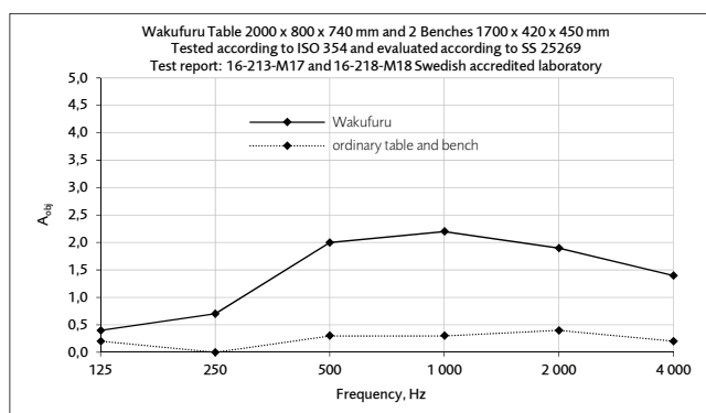
Equivalent absorption area per object (m²S/object)
